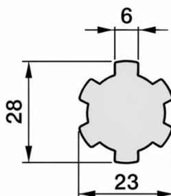
23 UNI221 Z=6
