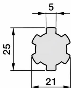
21 UNI221 Z=6
